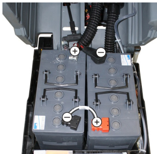
Installation sketch for 2 batteries
