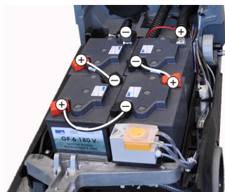
Installation sketch for 4 batteries
