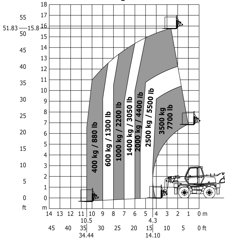
Laaddiagram
